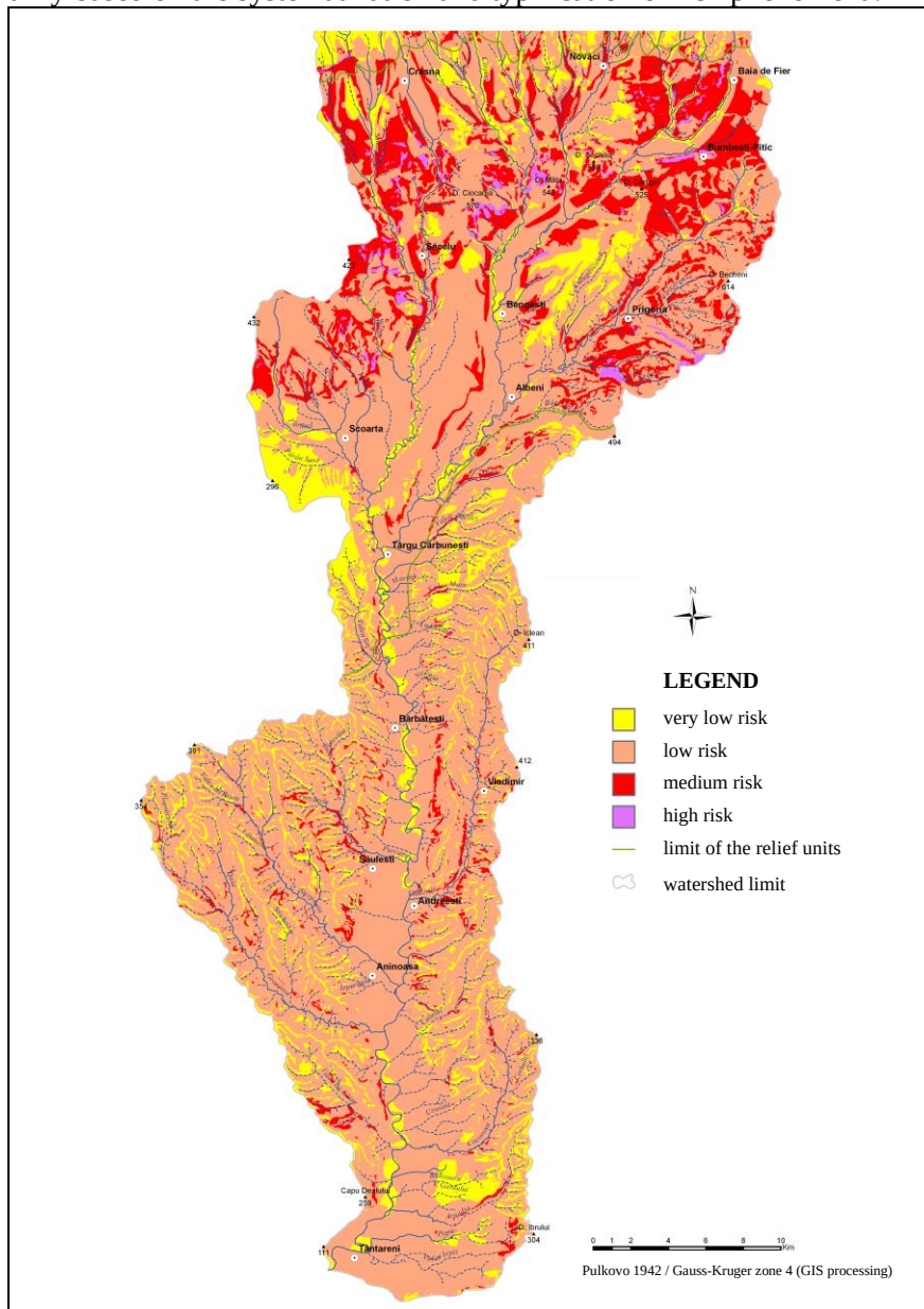
Fig. 2 The geomorphological risk map in the Subcarpathian and piedmont sector of the Gilort basin
