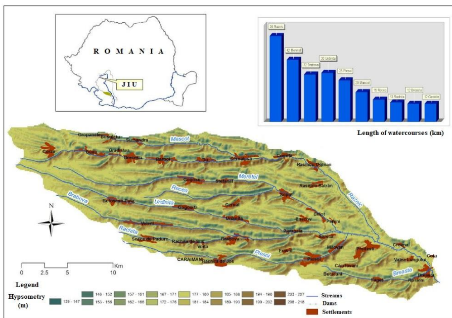
Fig. 1 Hypsometric map and hydrographic network – the Raznic river basin
