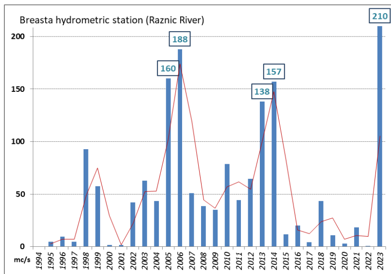
Fig. 2 Variation of the maximum annual flow recorded at Breasta hydrometric station
