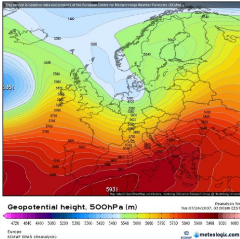
Fig. 10 The 500 hPa Geopotential height (reanalysis data ECMWF ERA5) (Source: https://meteologix.com )
