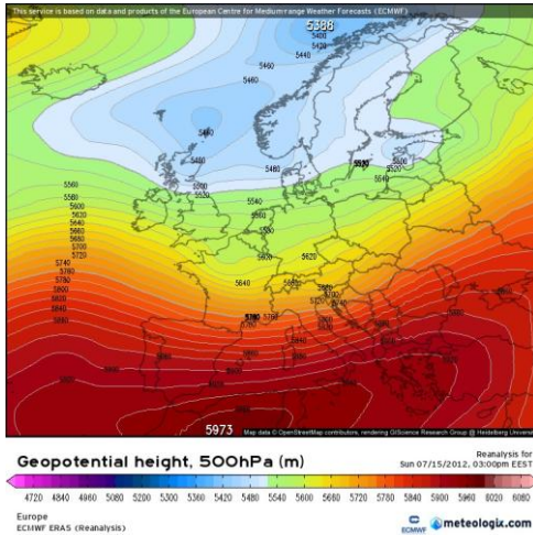
Fig. 13 The 500 hPa Geopotential height (reanalysis data ECMWF ERA5) at ground level on July 15, 2012, 12 UTC (Source: https://meteologix.com )
