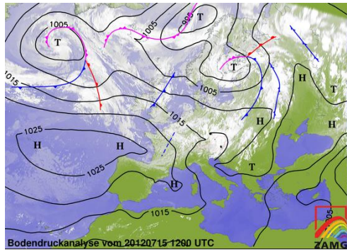
Fig. 14 Pressure and atmospheric fronts (Source: https://www.zamg.ac.at )
