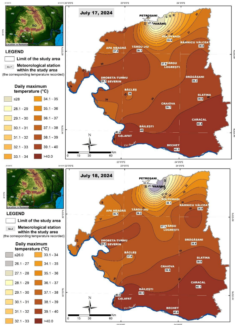
Fig. 2 Daily maximum temperatures registered on July 14, July 16-July 18
