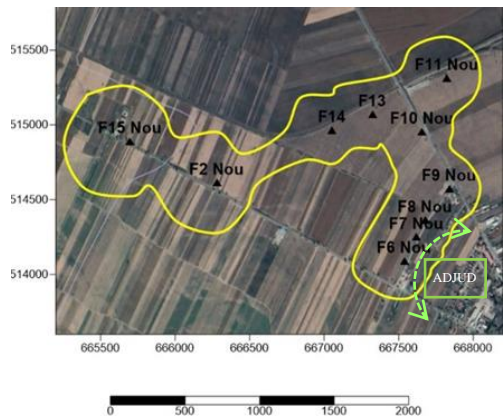
Fig. 4 50-day isochron - the delimitation of the protection zone for the 10 boreholes
